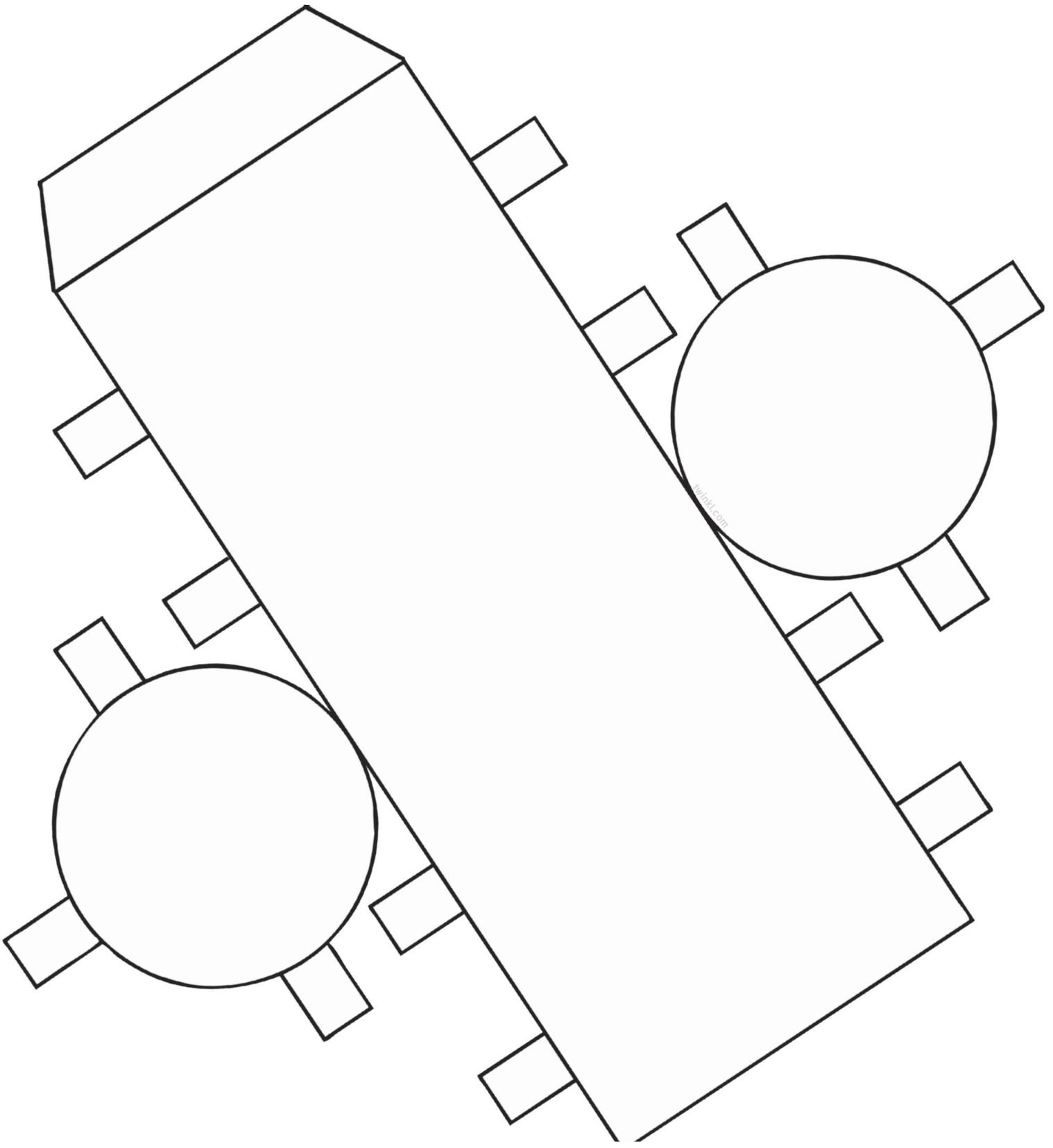
Cylinder
