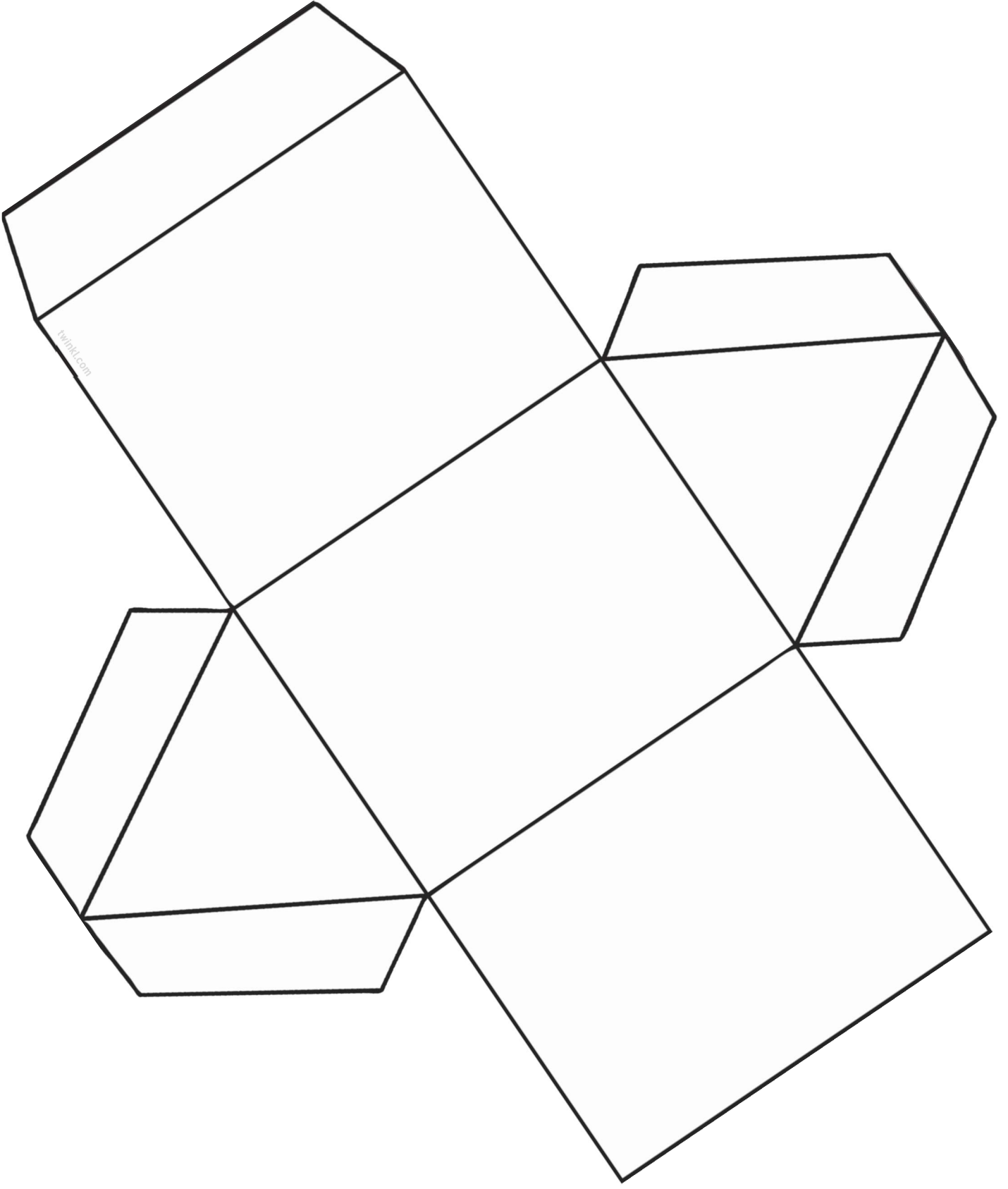
Triangular Prism
